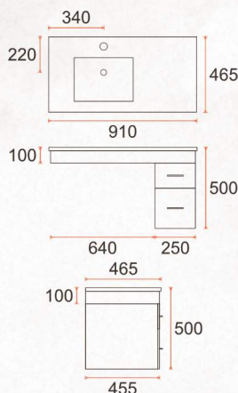
Accessible 900 Left Offset Basin
