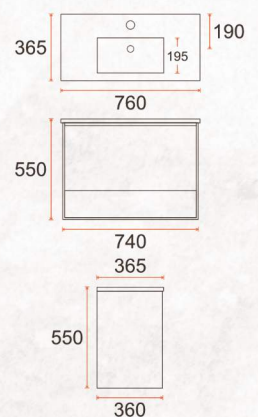
Galaxy 750 Slim - 365mm Basin Depth
