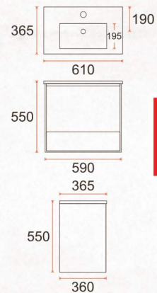
Galaxy 750 Slim - 365mm Basin Depth
