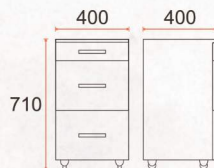
Castor Cabinet
